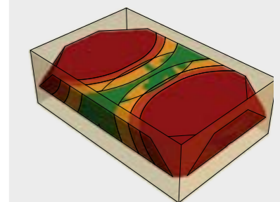
Heated effect with 2 sides heated (6 x 4 m format).
