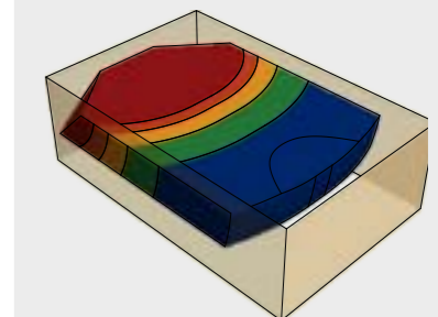
Heat effect with 1 side heated (6 x 4 m format)
